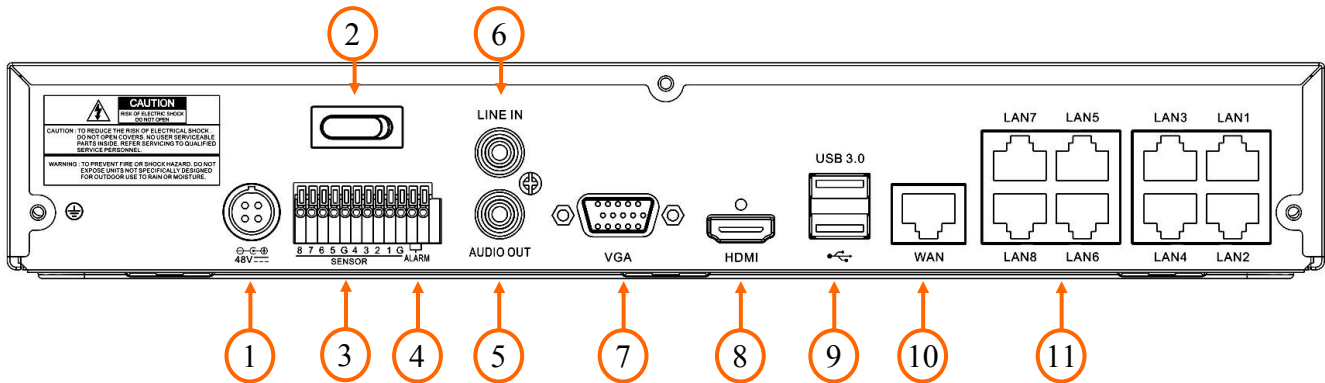
NVR-4308P8-H1
